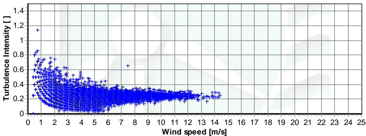
Figure 3 - Turbulence Intensity vs. Wind Speed, March 26, 2005- May 31, 2005.
