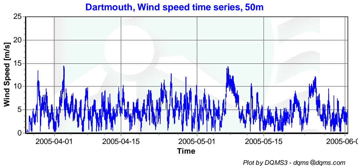
Figure 1- Wind Speed Time Series, March 26, 2005- May 31, 2005.
