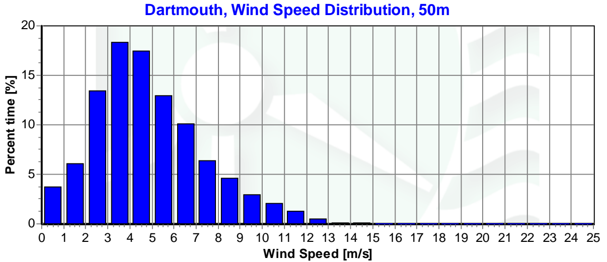
Figure 3 - Wind Speed Distribution, March 26, 2005- May 31, 2005.
