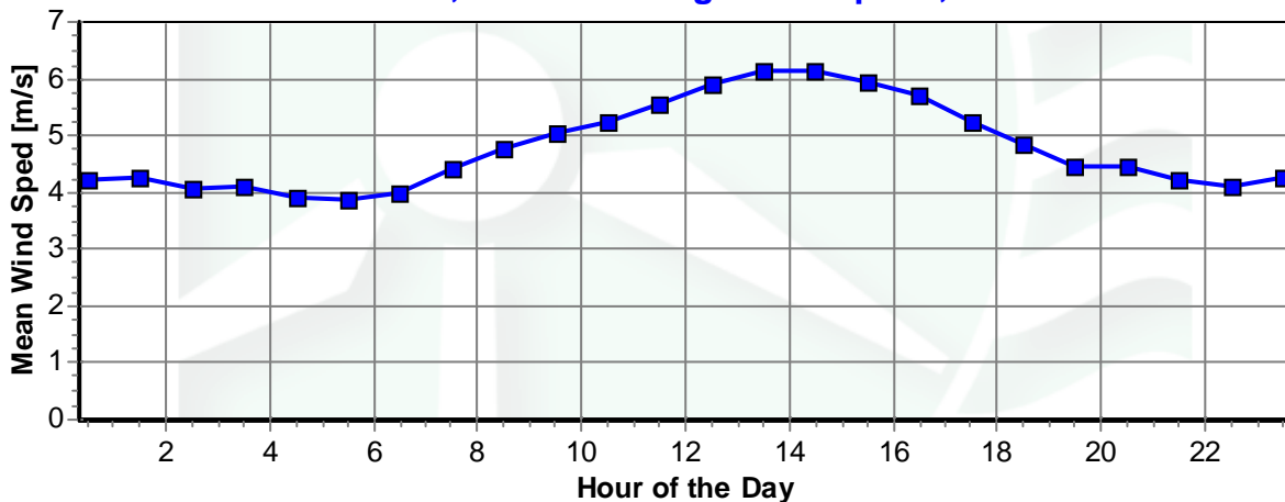
Figure 5 - Diurnal Wind Speed, March 26, 2005- May 31, 2005.
