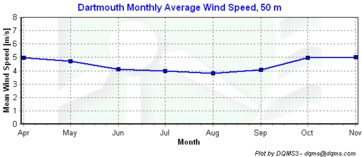
Figure 4 - Monthly average wind speeds, April 1, 2005 – November 30, 2005.
