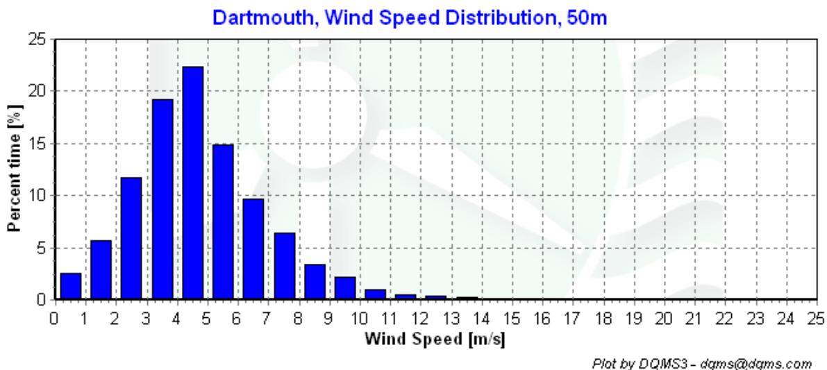
Figure 3 - Wind Speed Distribution, September 1, 2005 – November 30, 2005.
