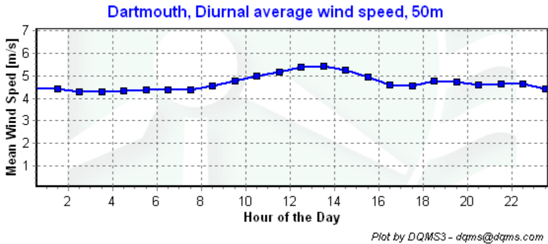
Figure 5 - Diurnal Wind Speed, September 1, 2005 – November 30, 2005.
