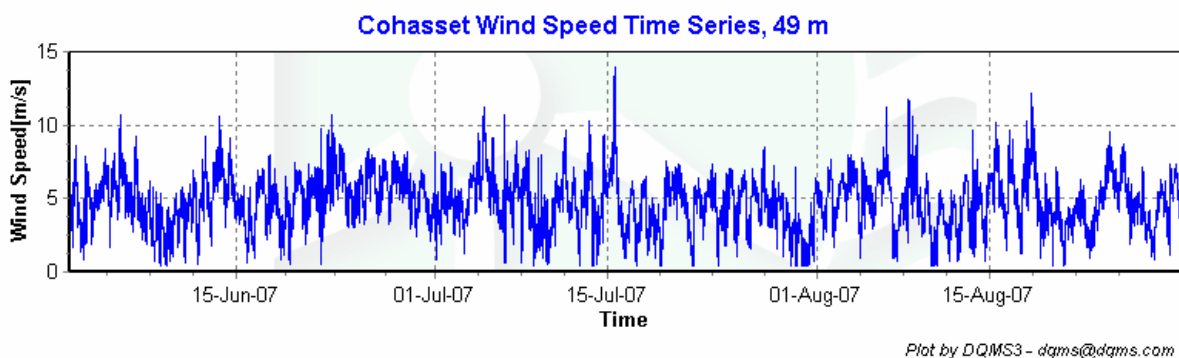
Figure 2 – Wind Speed Time Series, June 2007 – August 2007
