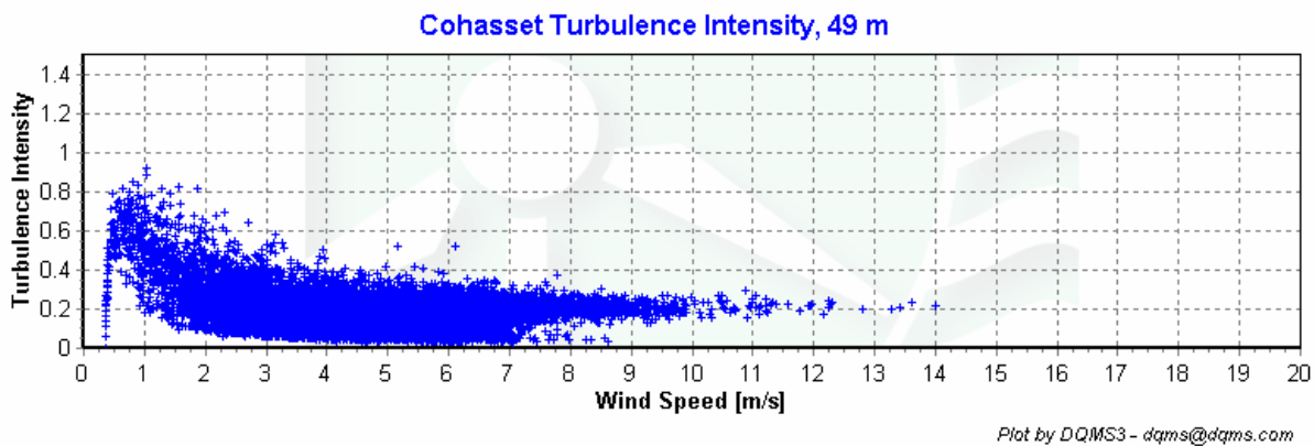
Figure 6 – Turbulence Intensity vs. Wind Speed, June 2007 – August 2007
