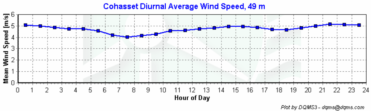
Figure 5 – Diurnal Wind Speed, June 2007 – August 2007
