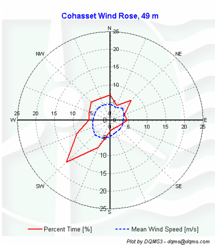
Figure 7 – Wind Rose, June 2007 – August 2007
