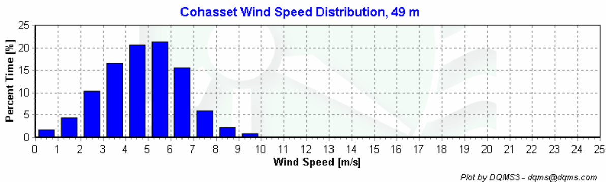
Figure 3 – Wind Speed Distribution, June 2007 – August 2007
