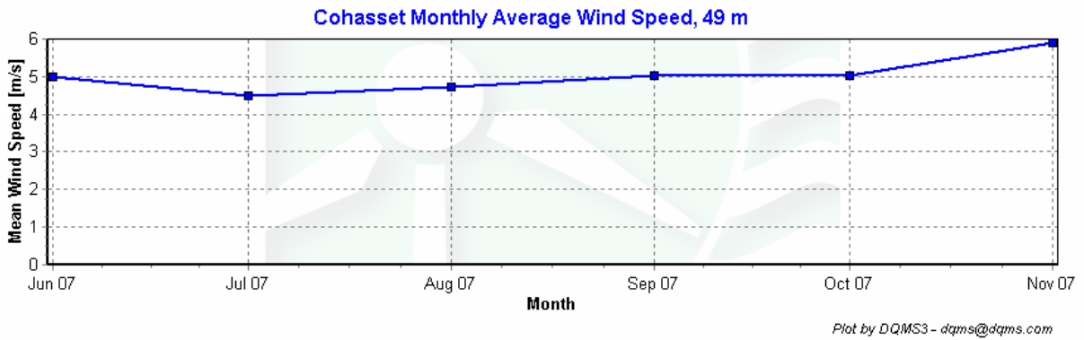
Figure 4 – Monthly Average Wind Speeds, June 2007 – November 2007
