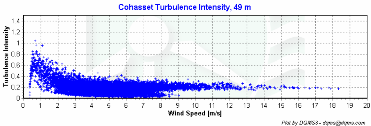
Figure 6 – Turbulence Intensity vs. Wind Speed, September 2007 – November 2007
