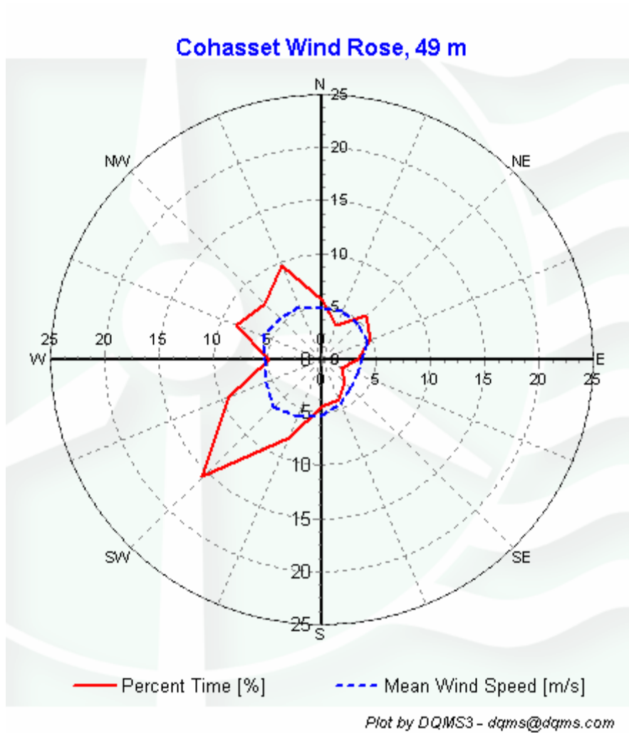
Figure 7 – Wind Rose, September 2007 – November 2007
