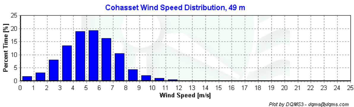
Figure 3 – Wind Speed Distribution, September 2007 – November 2007
