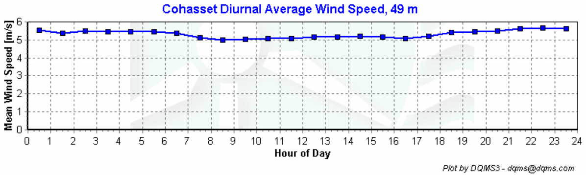
Figure 5 – Diurnal Wind Speed, September 2007 – November 2007
