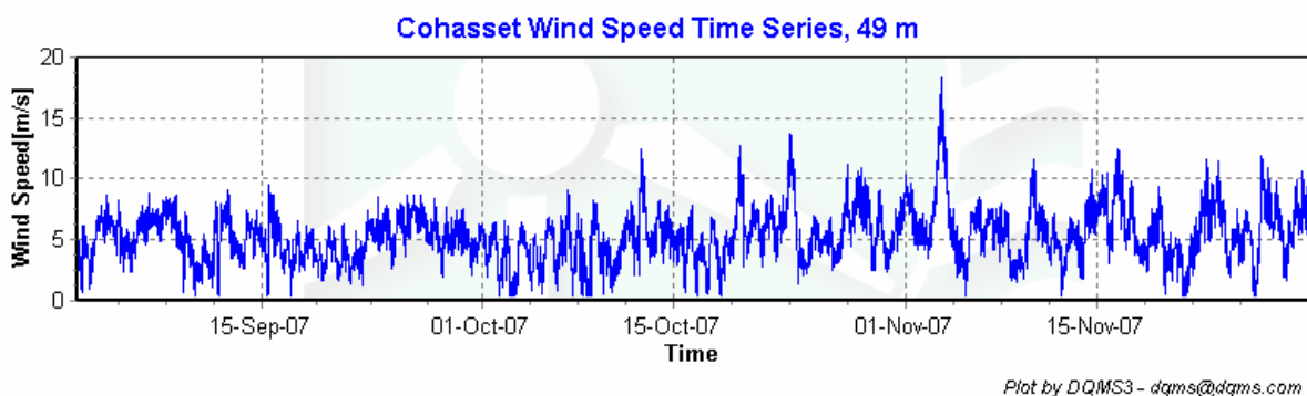
Figure 2 – Wind Speed Time Series, September 2007 – November 2007
