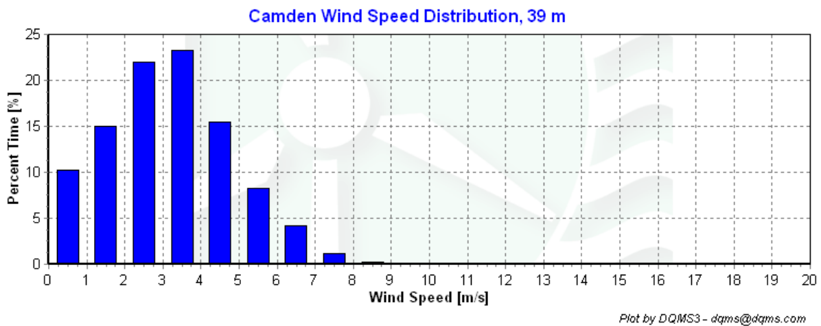
Figure 3 - Wind Speed Distribution, June 1, 2006 - August 31, 2006.
