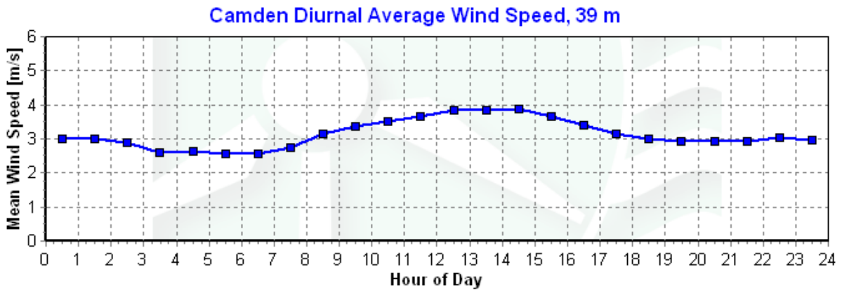
Figure 5 - Diurnal Wind Speed, June 1, 2006 - August 31, 2006.
