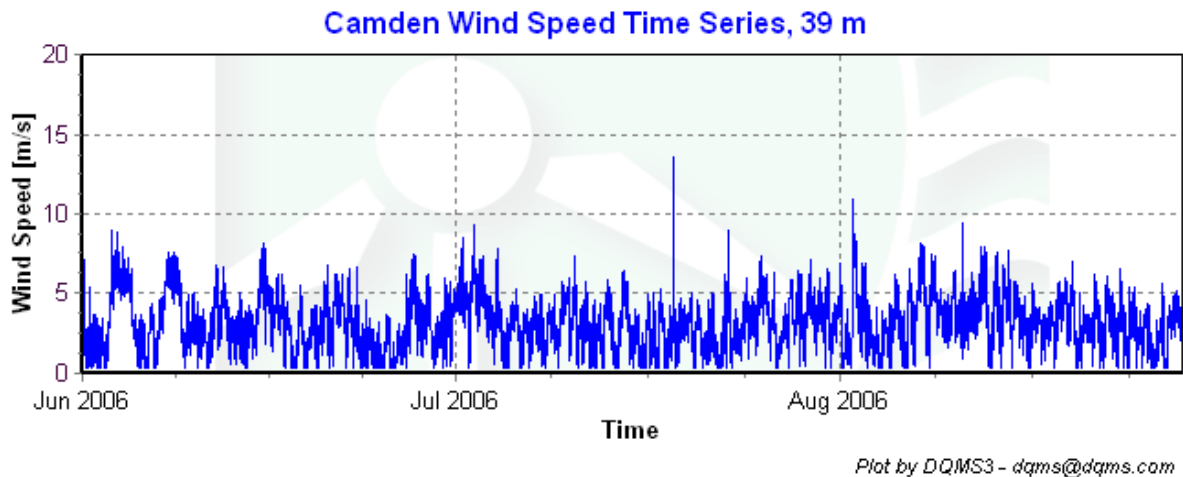
Figure 2 - Wind Speed Time Series, June 1, 2006 - August 31, 2006.
