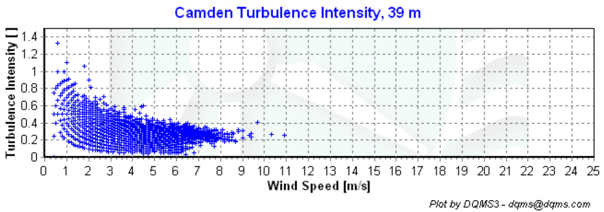
Figure 6 - Turbulence Intensity vs. Wind Speed, June 1, 2006 - August 31, 2006.
