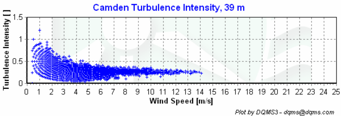
Figure 6 - Turbulence Intensity vs. Wind Speed, September 1, 2006 - November 30, 2006.
