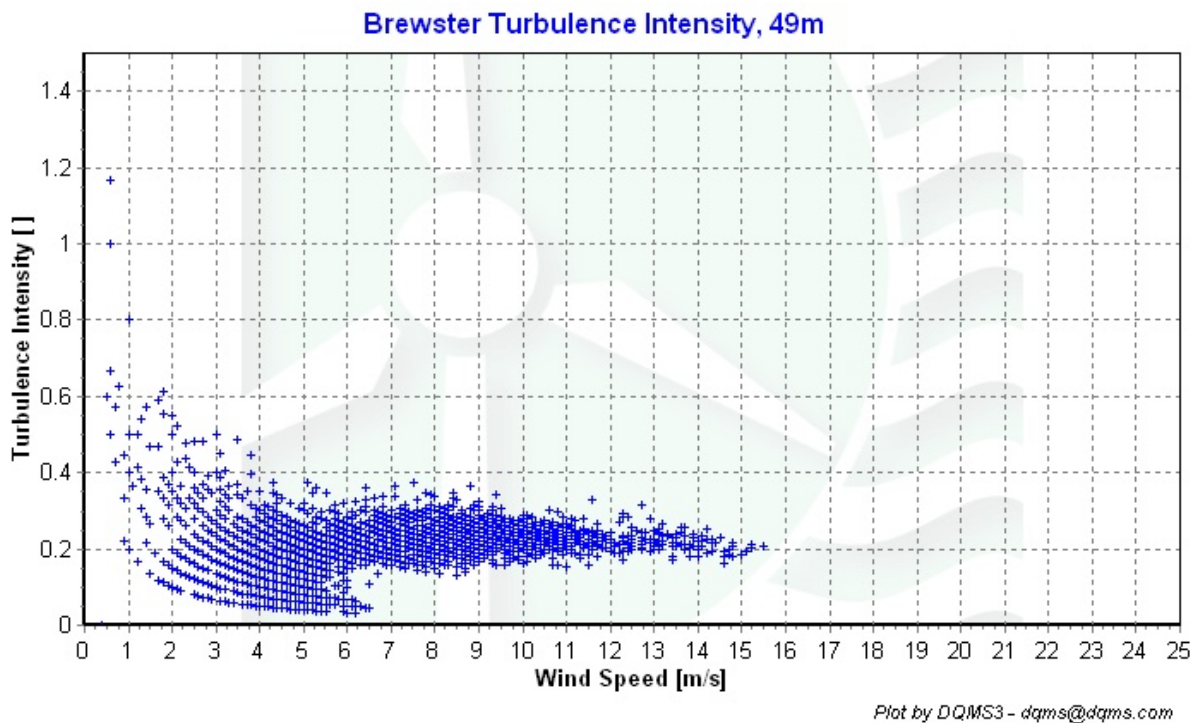
Figure 5 – Turbulence Intensity, Feb 1, 2006 through Feb 28, 2006
