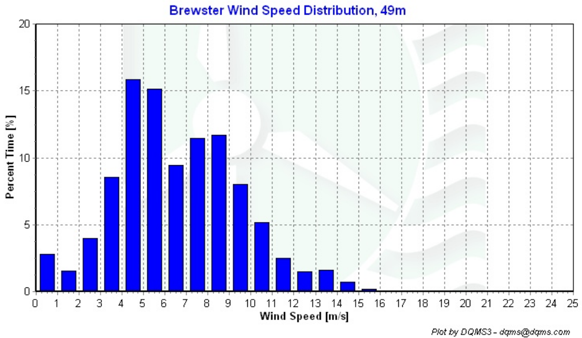
Figure 2 – Wind Speed Distribution, Feb 1, 2006 through Feb 28, 2006
