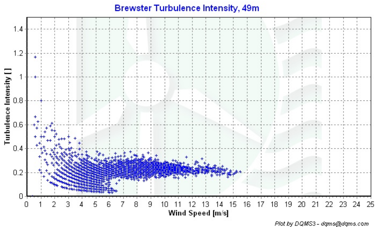
Figure 5 – Turbulence Intensity, Feb 1, 2006 through Feb 28, 2006
