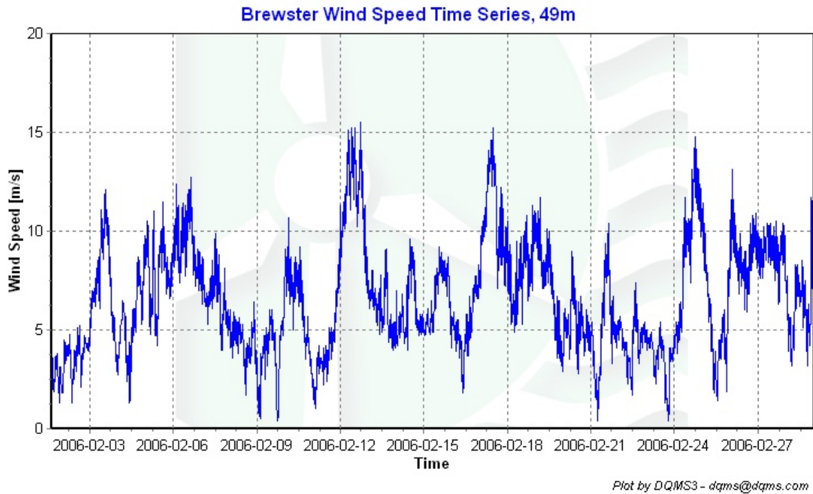
Figure 1 – Wind Speed Time Series, Feb 1, 2006 through Feb 28, 2006
