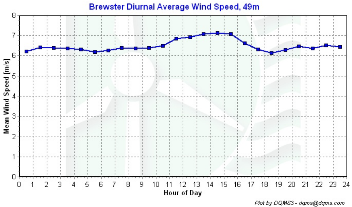
Figure 4 – Diurnal Average Wind Speed, Feb 1, 2006 through Feb 28, 2006
