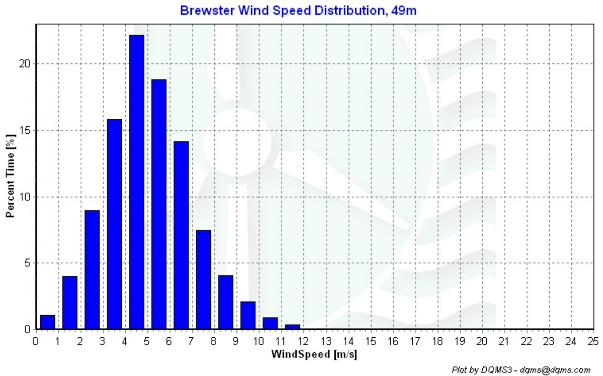
Figure 3 – Wind Speed Distribution, Jun 1 2006 through Aug 31 2006
