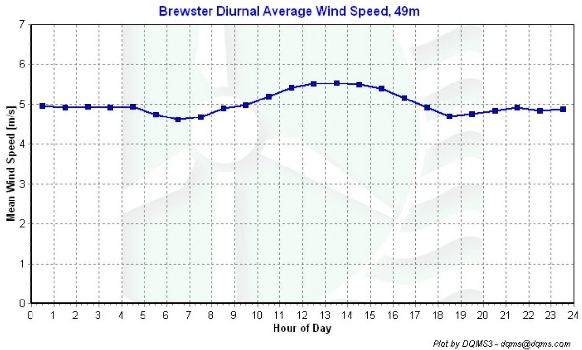
Figure 5 – Diurnal Average Wind Speed, Jun 1 2006 through Aug 31 2006
