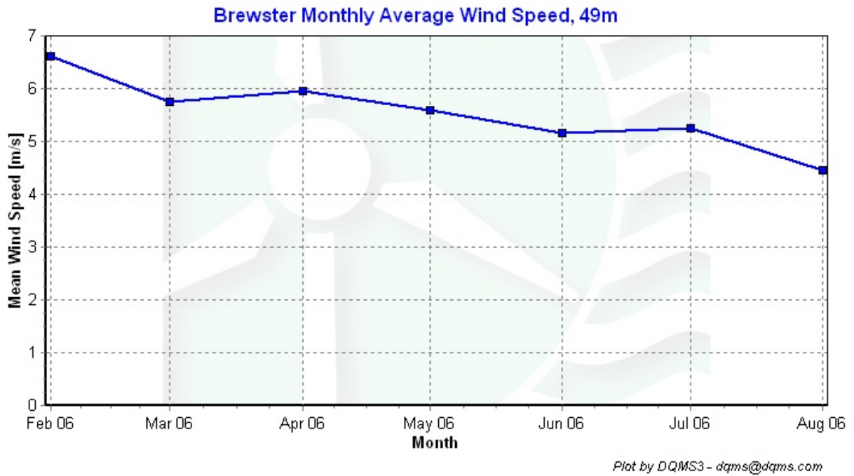
Figure 4 – Monthly Average Wind Speed, Feb 2006 to Aug 2006
