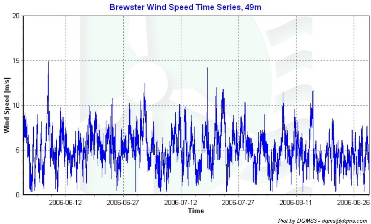
Figure 2 – Wind Speed Time Series, Jun 1 2006 through Aug 31 2006
