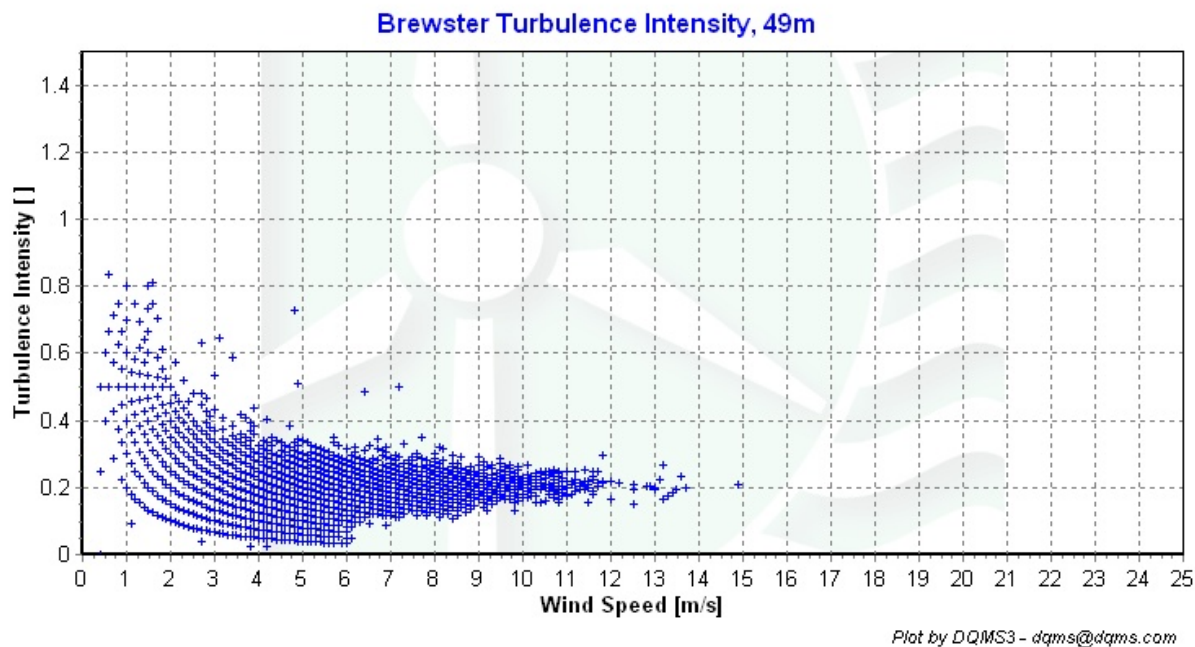
Figure 6 – Turbulence Intensity, Jun 1 2006 through Aug 31 2006
