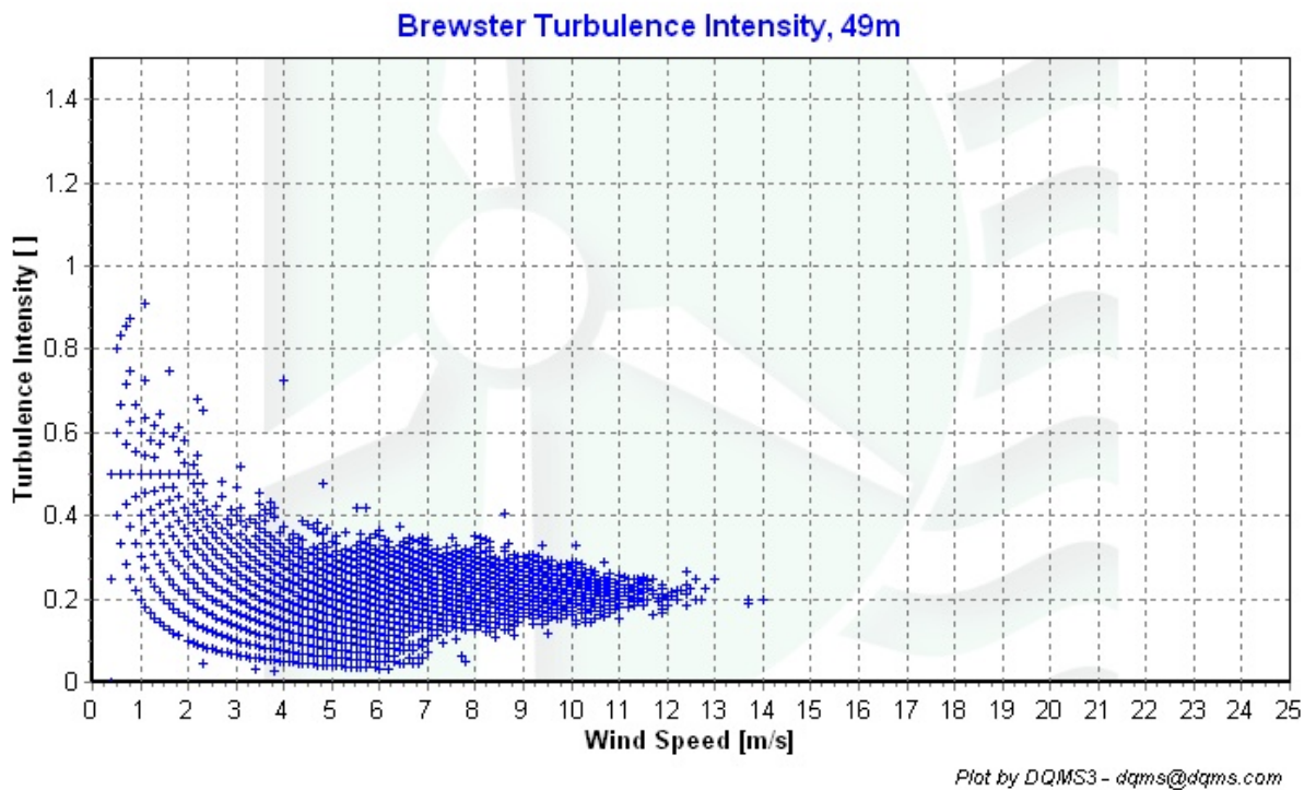
Figure 5 – Turbulence Intensity, Mar 1, 2006 through May 31, 2006
