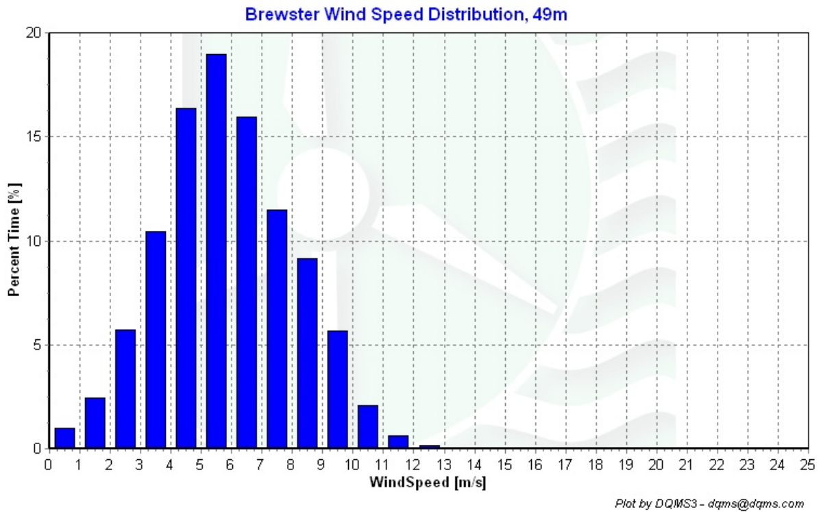
Figure 2 – Wind Speed Distribution, Mar 1, 2006 through May 31, 2006
