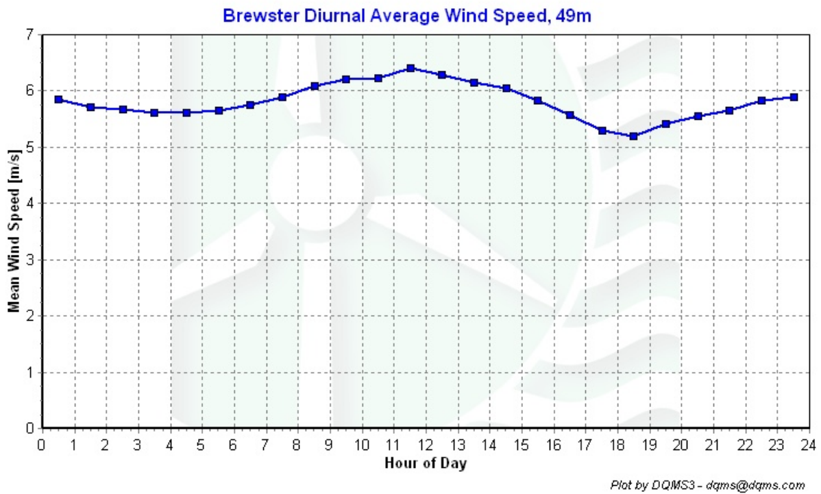
Figure 4 – Diurnal Average Wind Speed, Mar 1, 2006 through May 31, 2006
