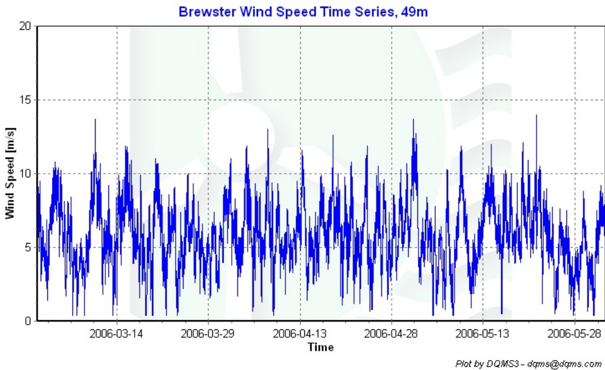
Figure 1 – Wind Speed Time Series, Mar 1, 2006 through May 31, 2006
