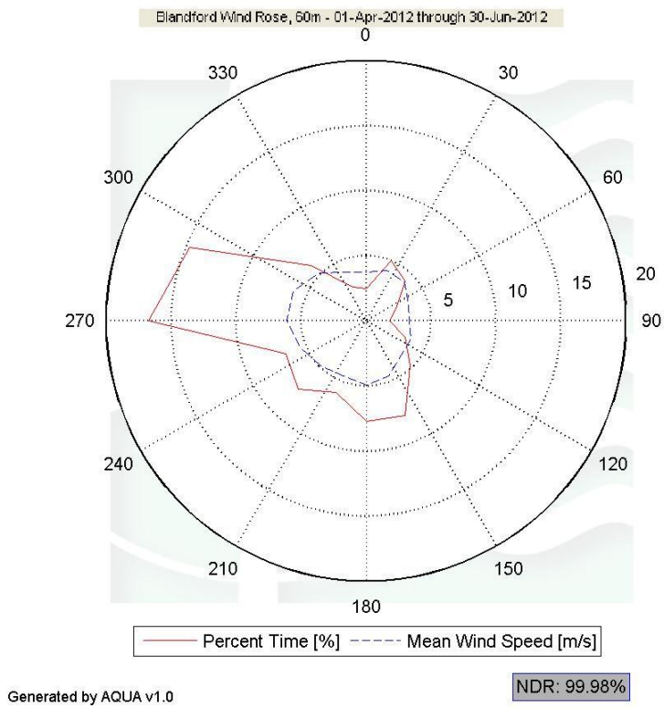
Figure 7 – Wind Rose, April 2012 - June 2012
