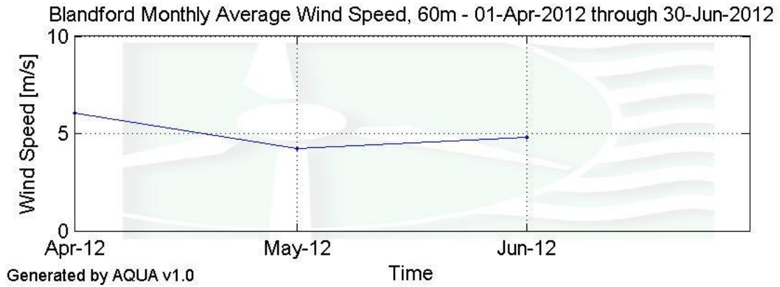
Figure 4 – Monthly Average Wind Speed, March 2012 - June 2012
