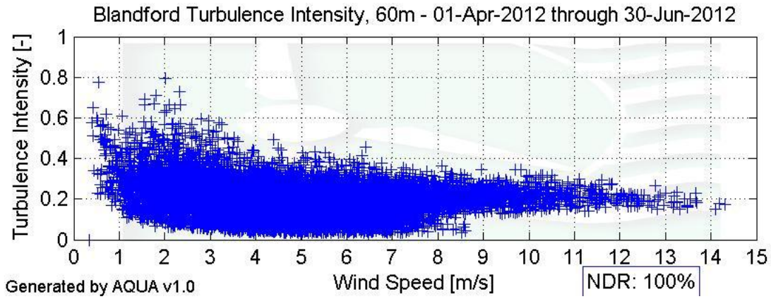
Figure 6 – Turbulence Intensity, April 2012 - June 2012
