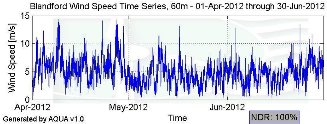
Figure 2 - Wind Speed Time Series, April 2012 - June 2012
