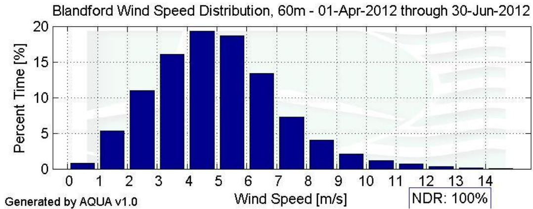
Figure 3 - Wind Speed Distribution, April 2012 - June 2012
