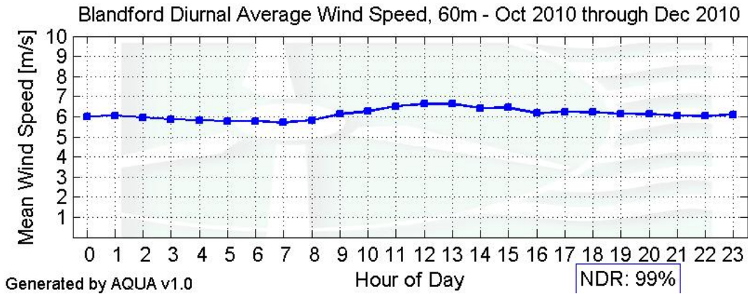
Figure 5 – Diurnal Average Wind Speed, October – December 2010
