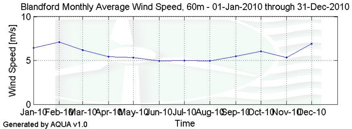
Figure 4 – Monthly Average Wind Speed, October – December 2010
