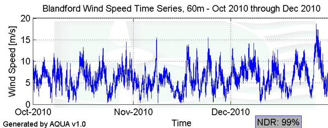
Figure 2 - Wind Speed Time Series, October – December 2010
