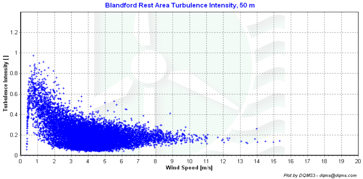
Figure 6 – Turbulence Intensity vs. Wind Speed, June 1, 2008 – August 31, 2008
