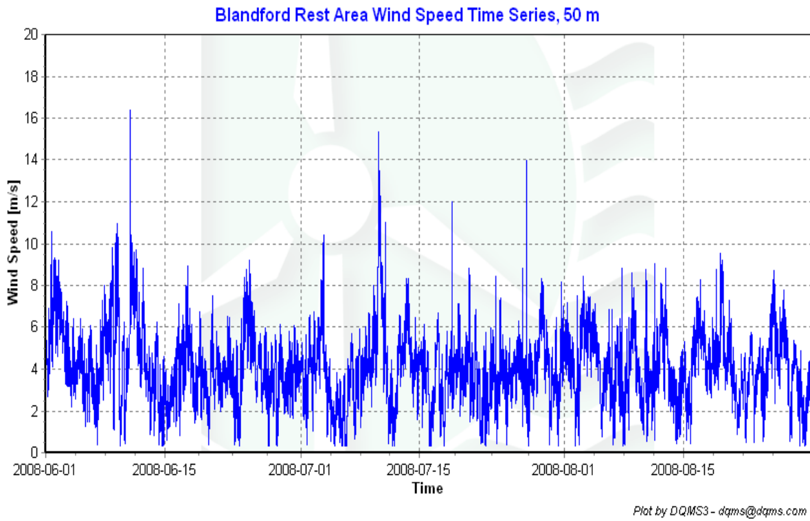
Figure 2 – Wind Speed Time Series, June 1, 2008 – August 31, 2008
