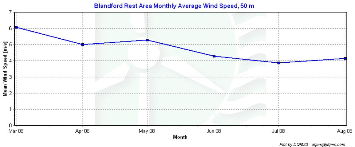
Figure 4 – Monthly Average Wind Speed, June 1, 2008 – August 31, 2008
