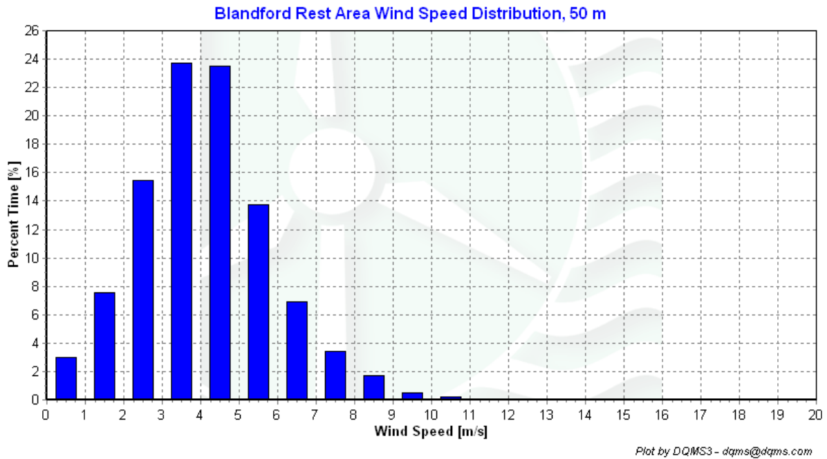
Figure 3 – Wind Speed Distribution, June 1, 2008 – August 31, 2008
