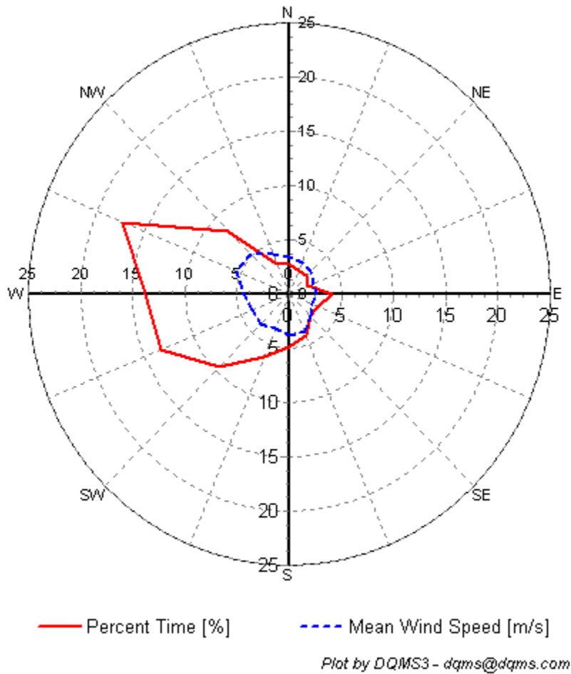
Figure 7 – Wind Rose, June 1, 2008 – August 31, 2008
