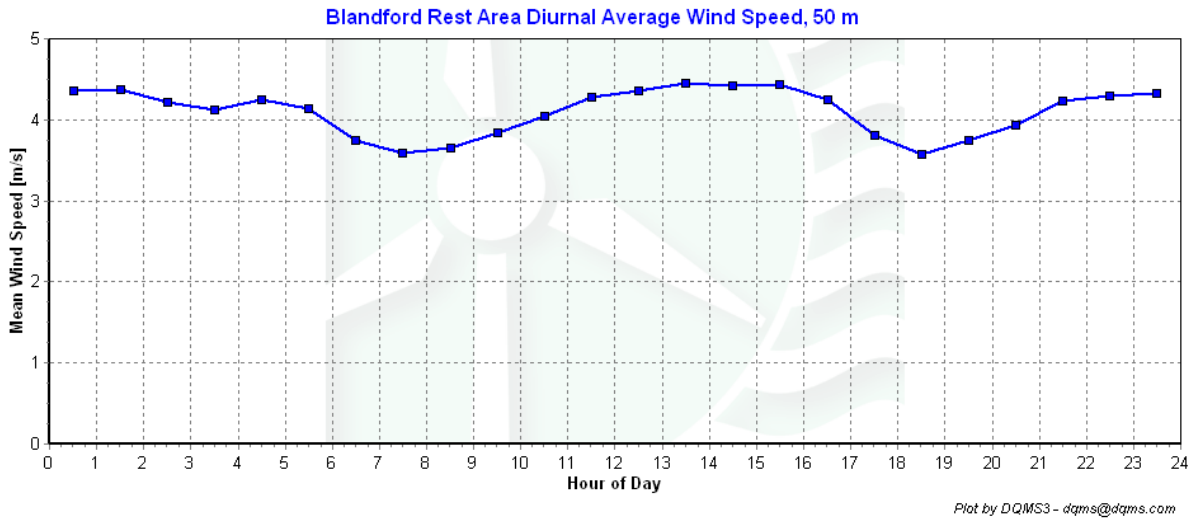
Figure 5 – Diurnal Average Wind Speeds, June 1, 2008 – August 31, 2008
