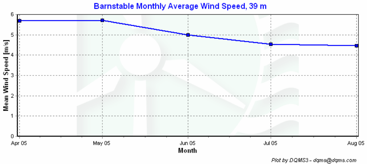
Figure 4 – Barnstable monthly average wind speed, April – August 2005
