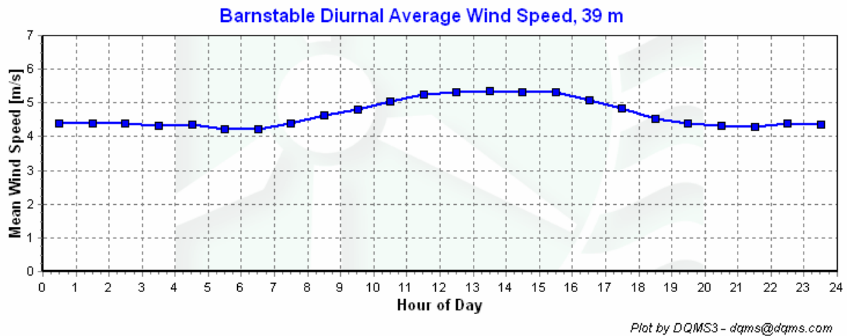
Figure 5 – Barnstable diurnal average wind speed, June 1 – August 31, 2005
