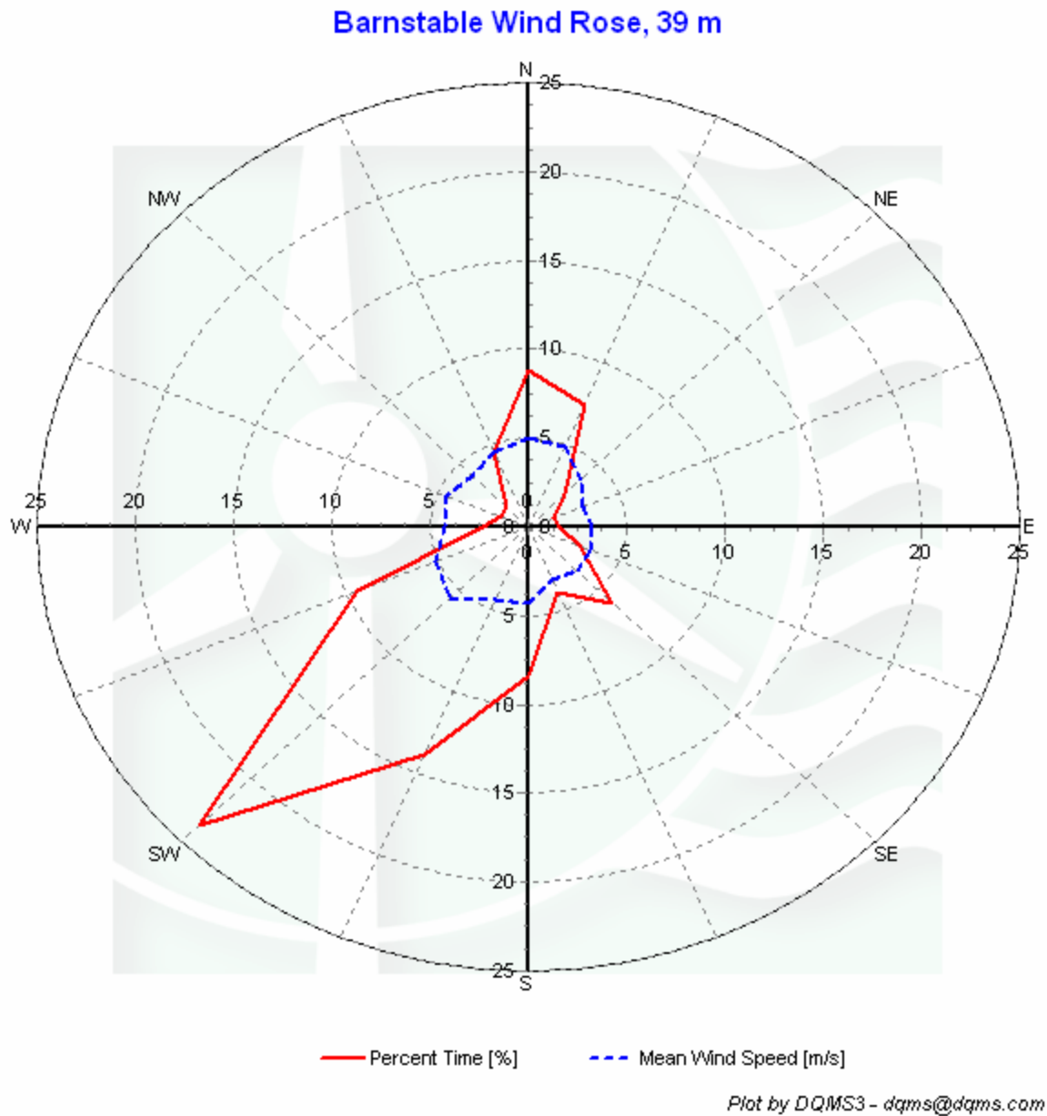
Figure 7 – Barnstable wind rose, June 1 – August 31, 2005
