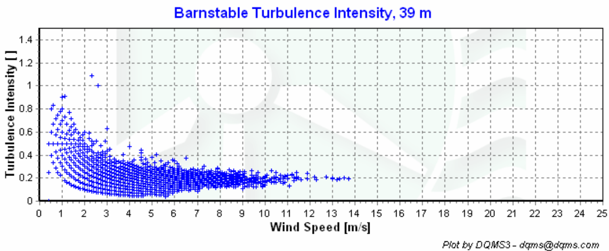
Figure 6 – Barnstable turbulence intensity, June 1 – August 31, 2005
