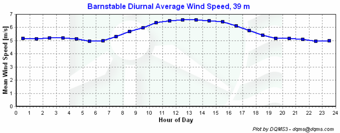
Figure 5 – Barnstable diurnal average wind speed, April 1 – May 31, 2005
