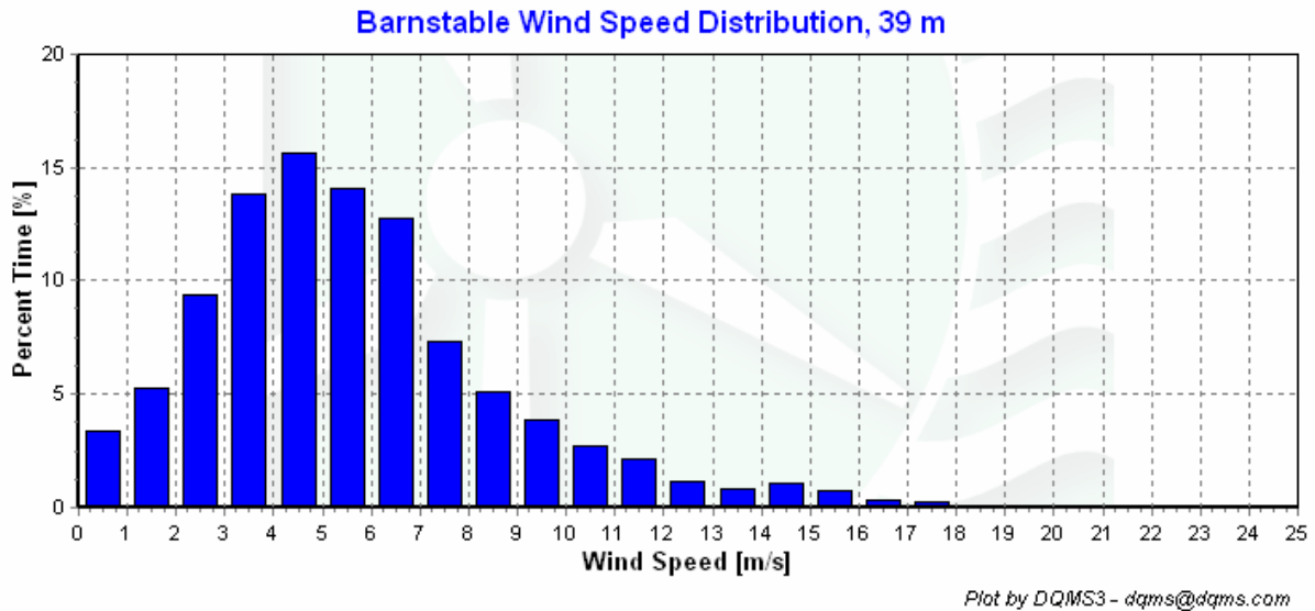
Figure 3 – Barnstable wind speed distribution, April 1 – May 31, 2005
