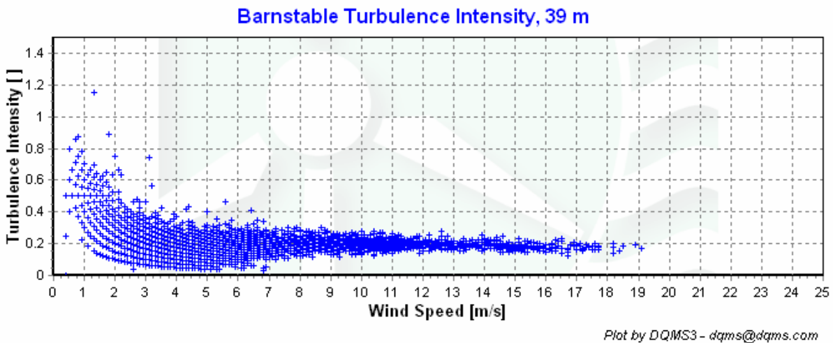
Figure 6 – Barnstable turbulence intensity, April 1 – May 31, 2005
