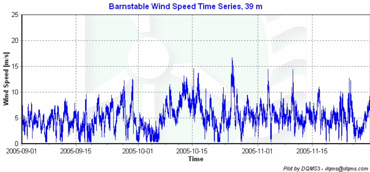
Figure 2 – Barnstable wind speed time series, September 1 – November 31, 2005
