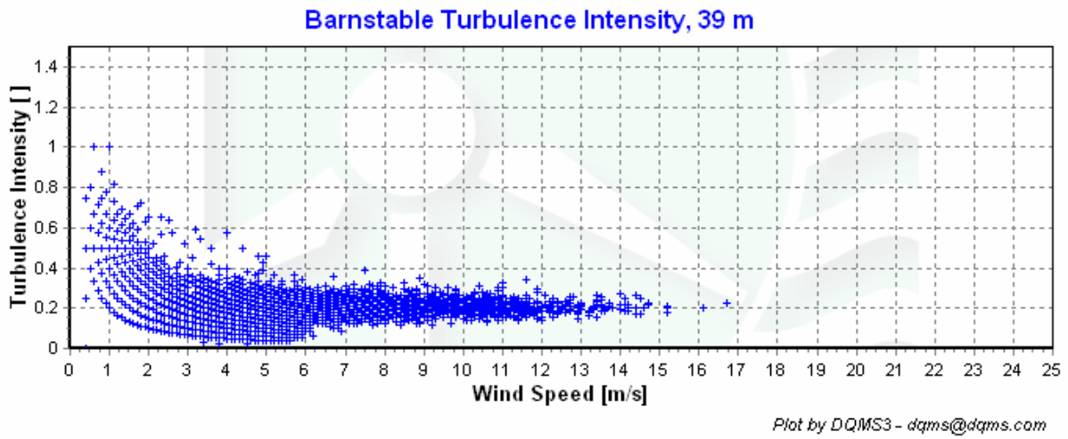
Figure 6 – Barnstable turbulence intensity, September 1 – November 31, 2005
