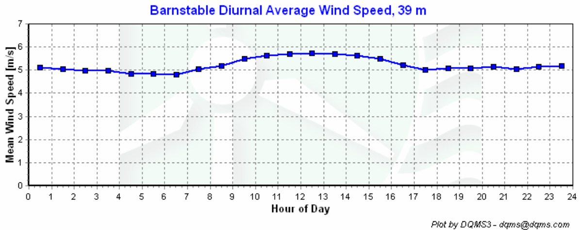
Figure 5 – Barnstable diurnal average wind speed, September 1 – November 31, 2005
