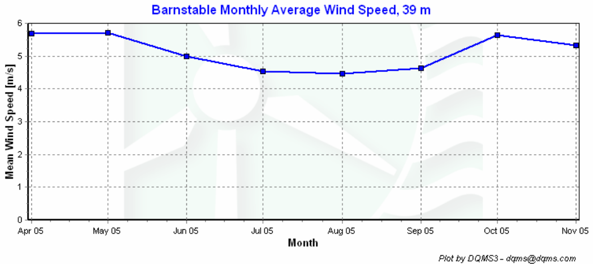
Figure 4 – Barnstable monthly average wind speed, April – November 2005
