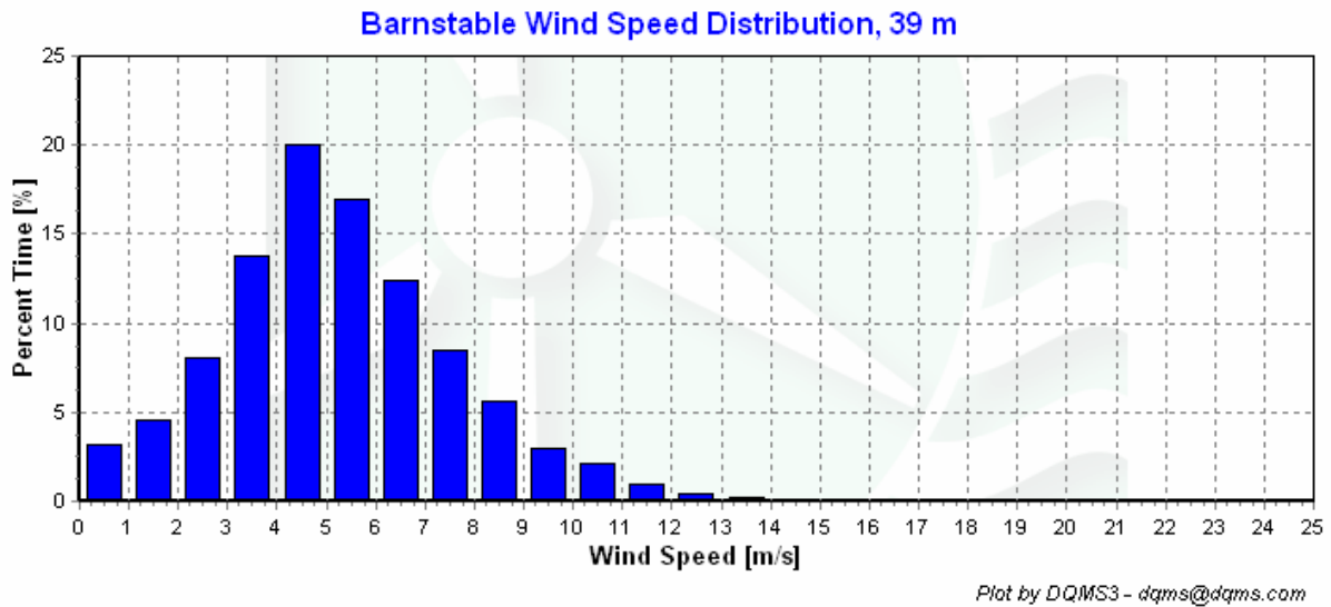
Figure 3 – Barnstable wind speed distribution, September 1 – November 31, 2005
