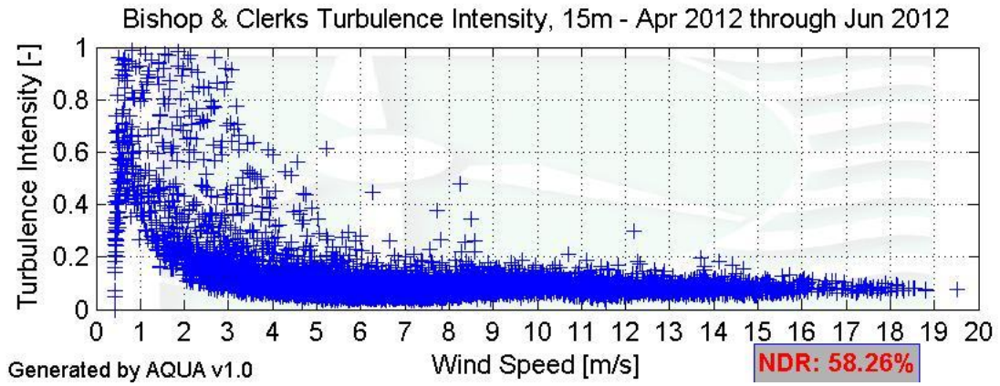
Figure 7 – Turbulence Intensity
