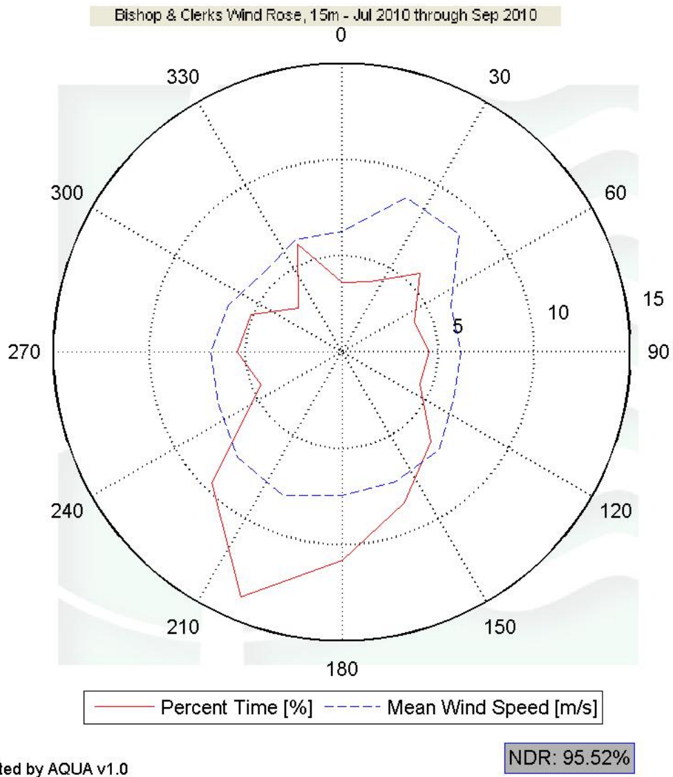
Figure 9 – Wind Rose
