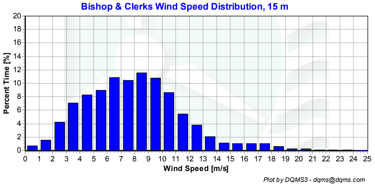
Figure 5 - Wind Speed Distribution, December 2004 – February 2005
