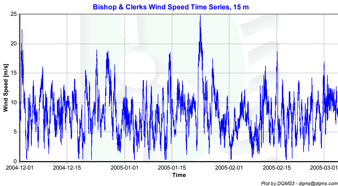
Figure 4 - Wind Speed Time Series, December 2004 – February 2005
