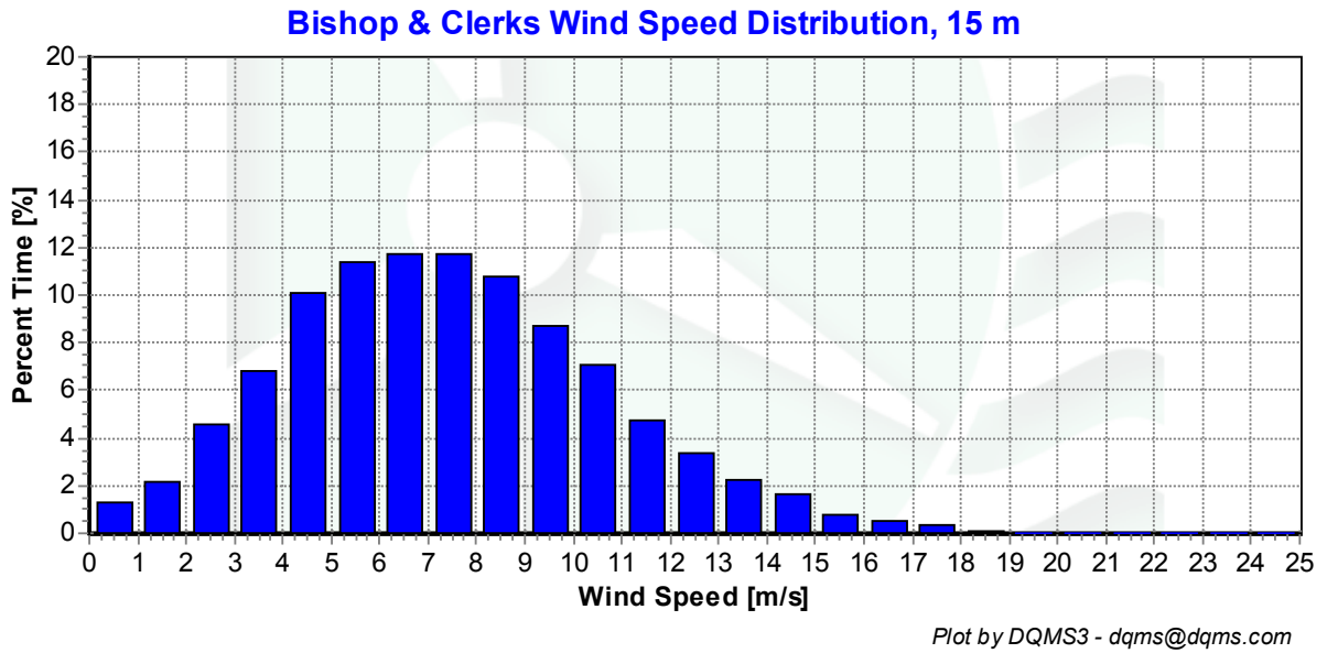
Figure 5 - Wind Speed Distribution, March 2004 – May 2004
