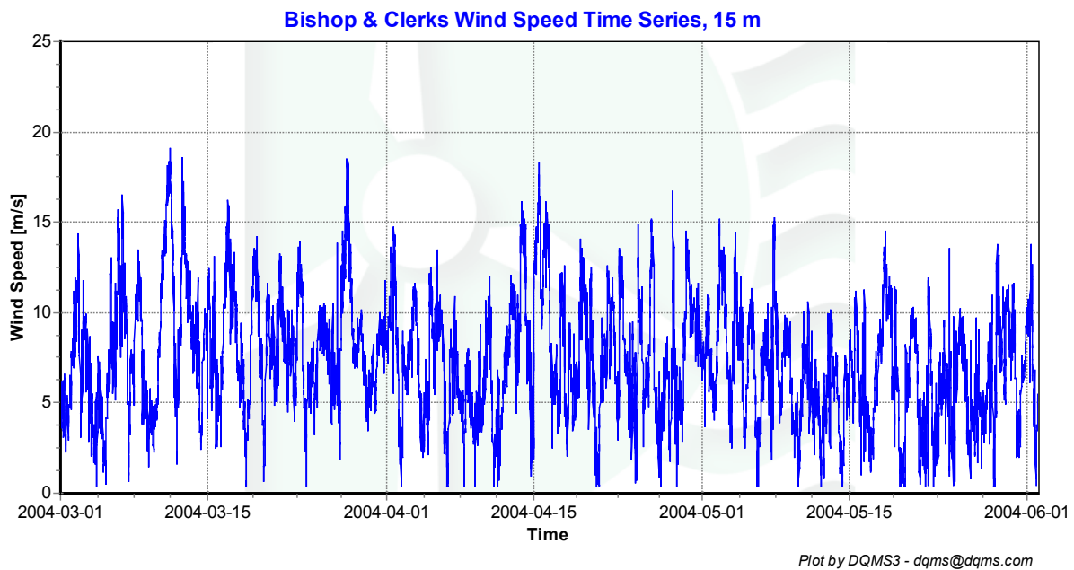
Figure 4 - Wind Speed Time Series, March 2004 – May 2004
