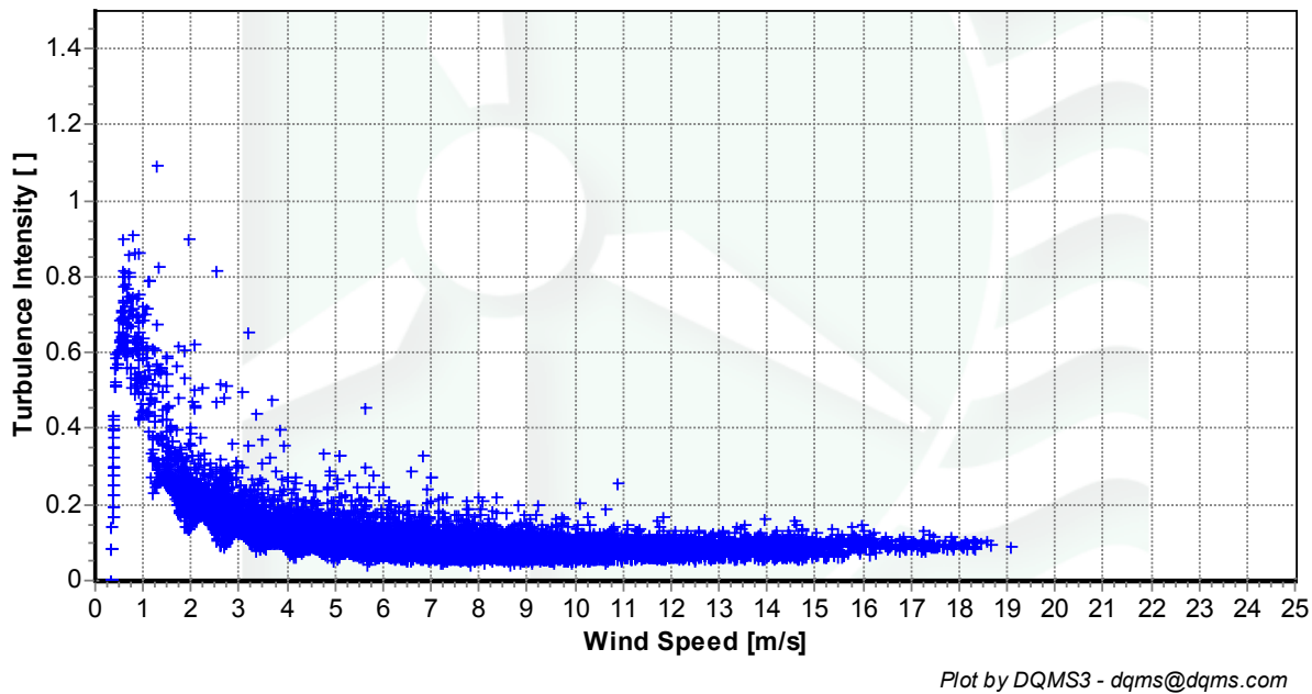
Figure 8 - Turbulence Intensity vs Wind Speed, March 2004 – May 2004
