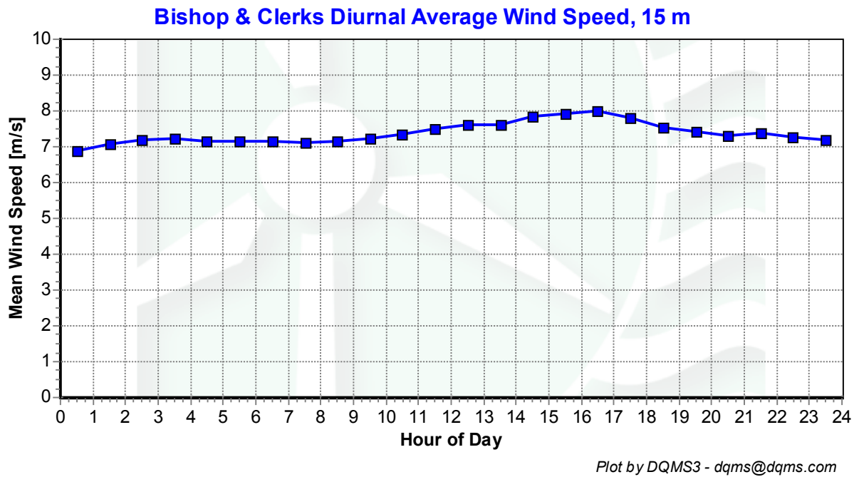
Figure 7 - Diurnal Wind Speed, March 2004 – May 2004
