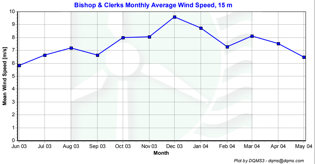
Figure 6 - Monthly average wind speed
