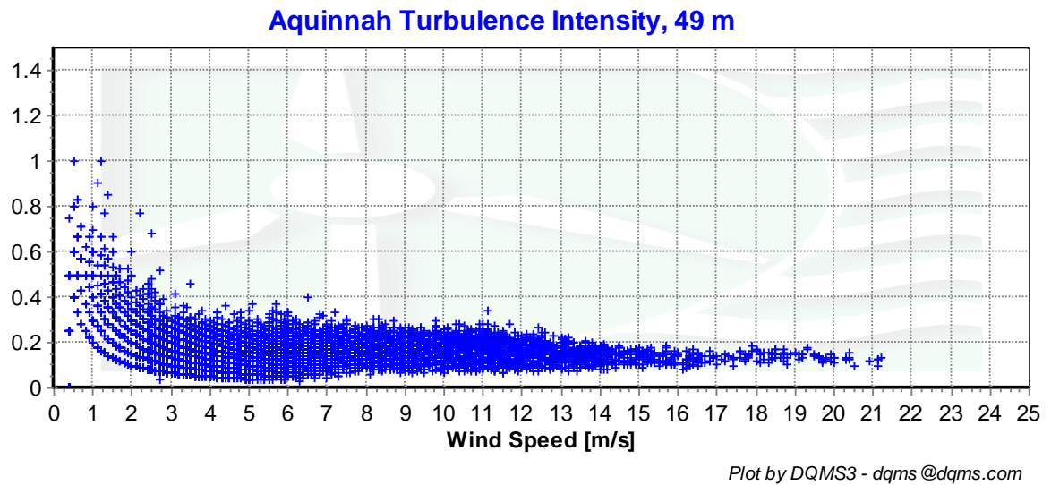
Figure 6 – Turbulence Intensity vs. Wind Speed, September 1, 2008 – November 31, 2008
