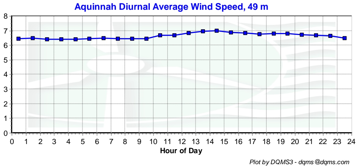
Figure 5 – Diurnal Average Wind Speeds, September 1, 2008 – November 31, 2008
