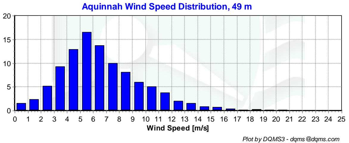
Figure 3 – Wind Speed Distribution, September 1, 2008 – November 31, 2008
