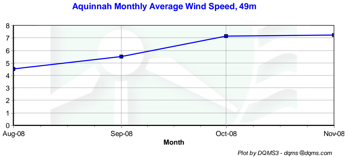
Figure 4 – Monthly Average Wind Speed, August 1, 2008 – November 31, 2008
