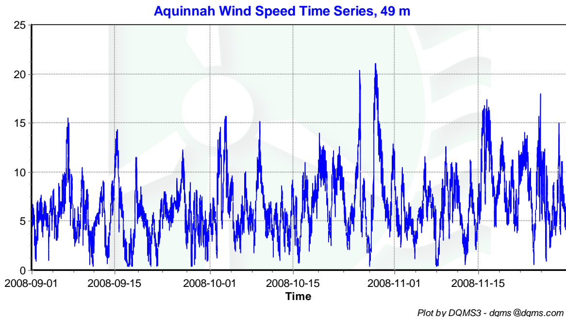
Figure 2 – Wind Speed Time Series, September 1, 2008 – November 31, 2008
