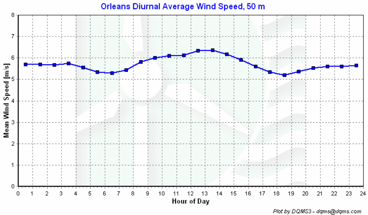
Figure 5 - Diurnal Wind Speed, March 2005 - May 2005
