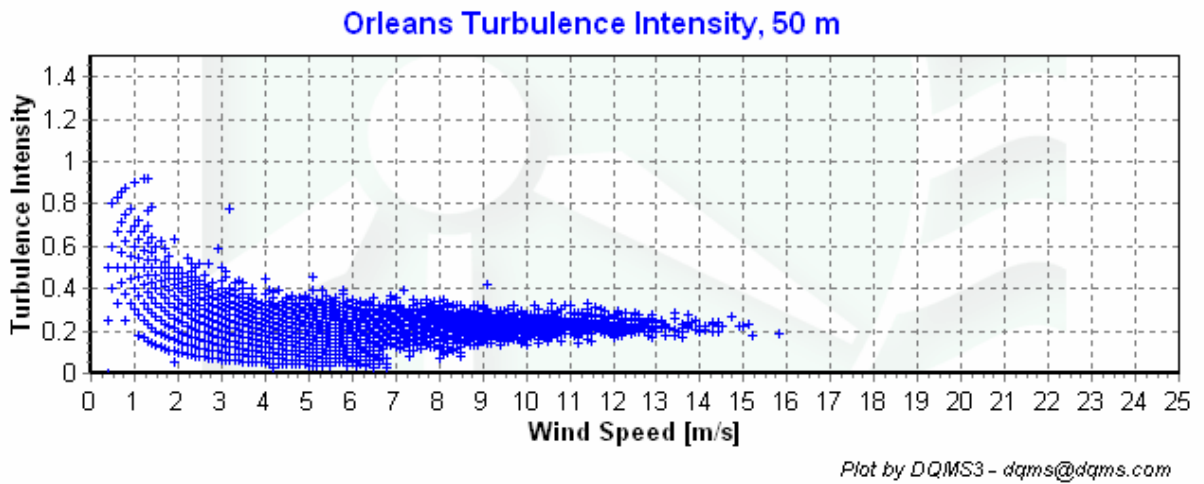
Figure 6 - Turbulence Intensity vs. Wind Speed, March 2004 - May 2005
