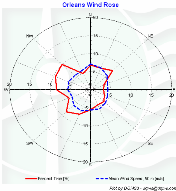
Figure 7 - Wind Rose, March 2005 - May 2005
