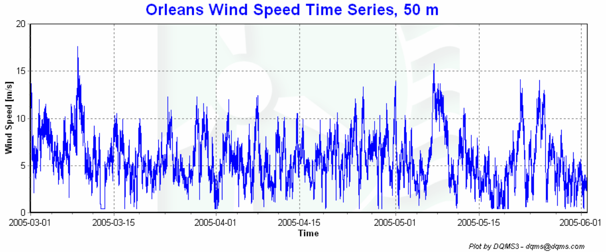
Figure 2 - Wind Speed Time Series, March 2005 - May 2005
