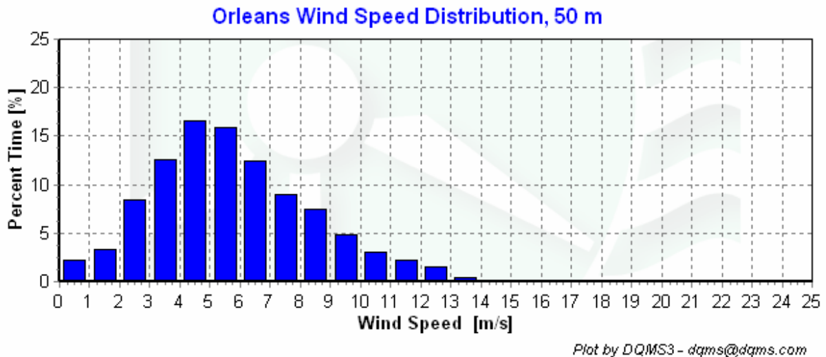
Figure 3 - Wind Speed Distribution, March 2005 - May 2005
