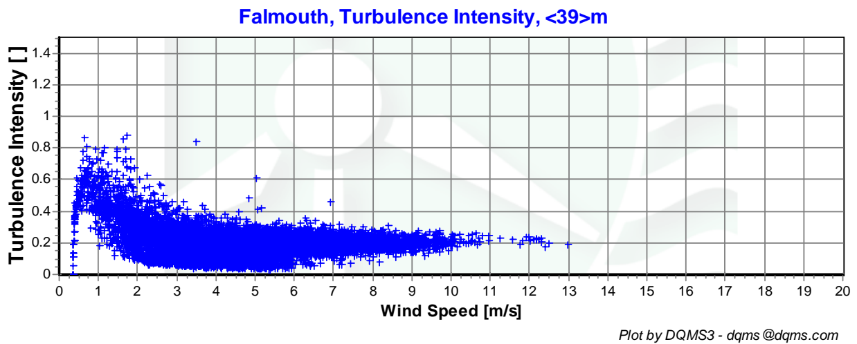
Figure 6 - Turbulence Intensity vs. Wind Speed, June 2004- Aug 2004
