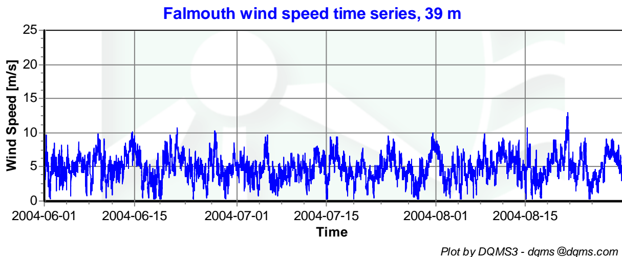
Figure 2- Wind Speed Time Series, June1, 2004 to August 31, 2004
