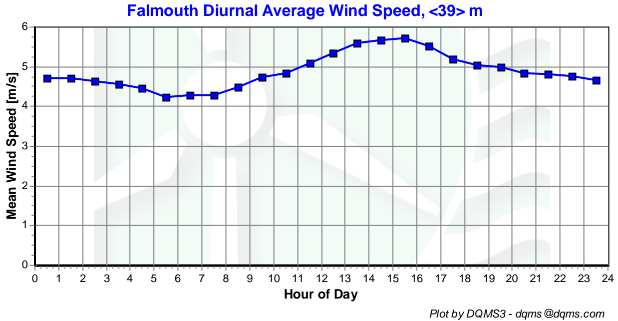
Figure 5 - Diurnal Wind Speed, June 2004- Aug 2004
