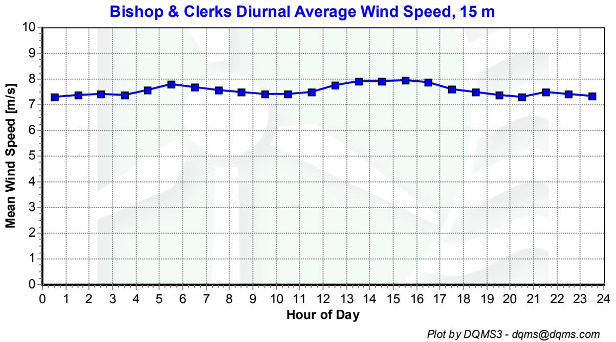
Figure 7 - Diurnal Wind Speed, September 2003 – November 2003
