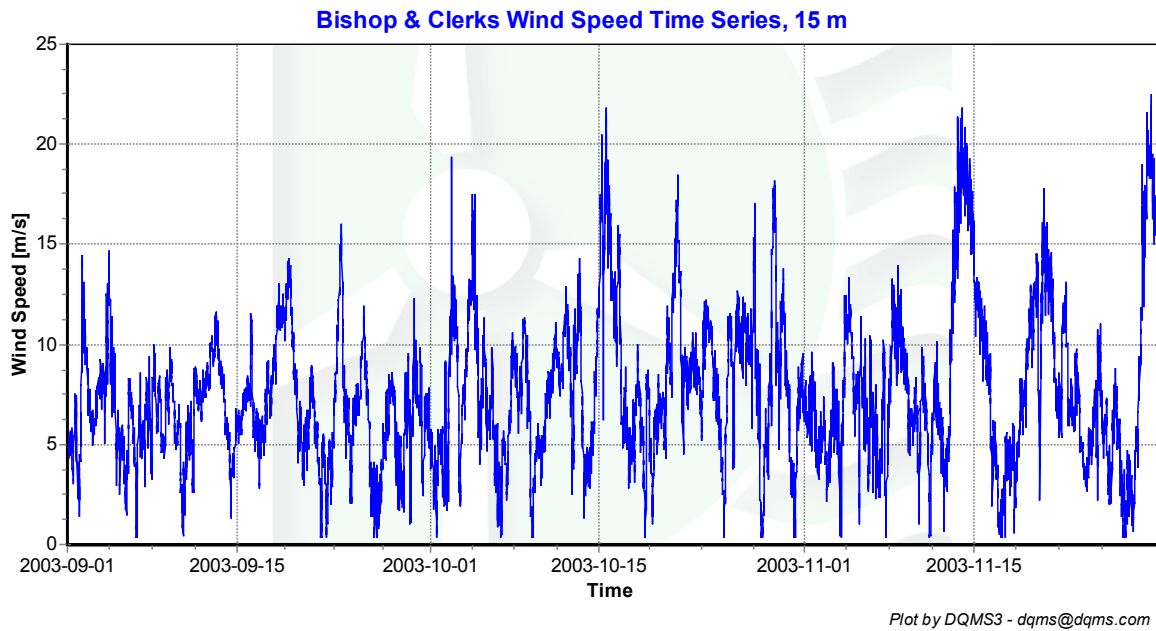
Figure 4 - Wind Speed Time Series, September 2003 – November 2003
