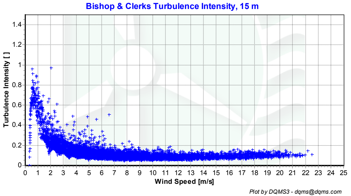
Figure 8 - Turbulence Intensity vs Wind Speed, September 2003 – November 2003
