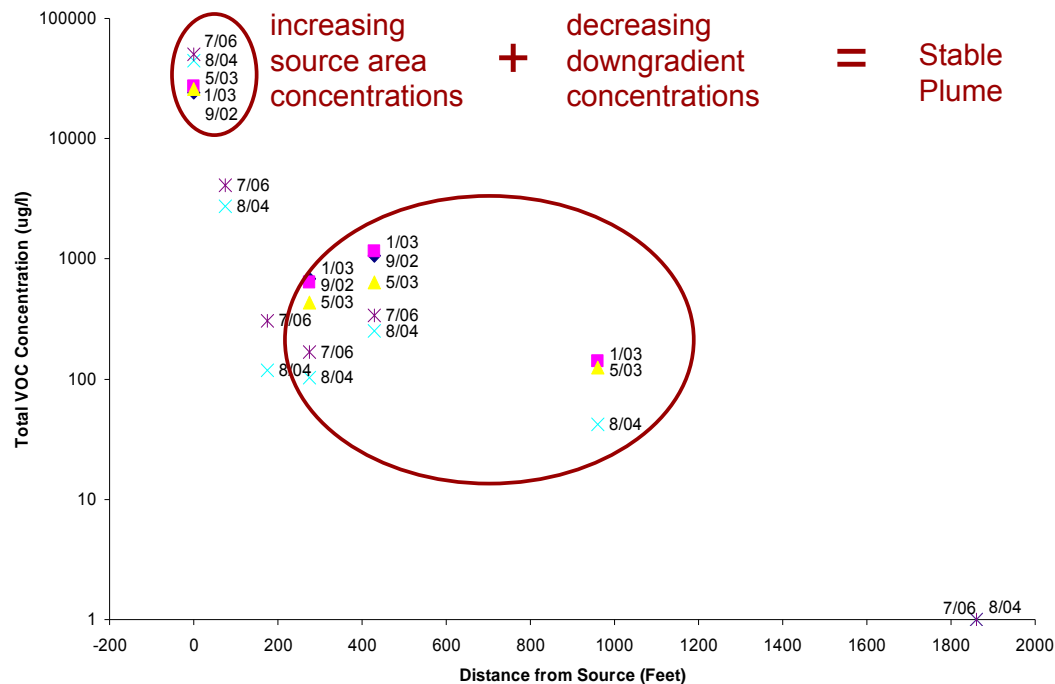
Total VOC Trend with Time and Distance
