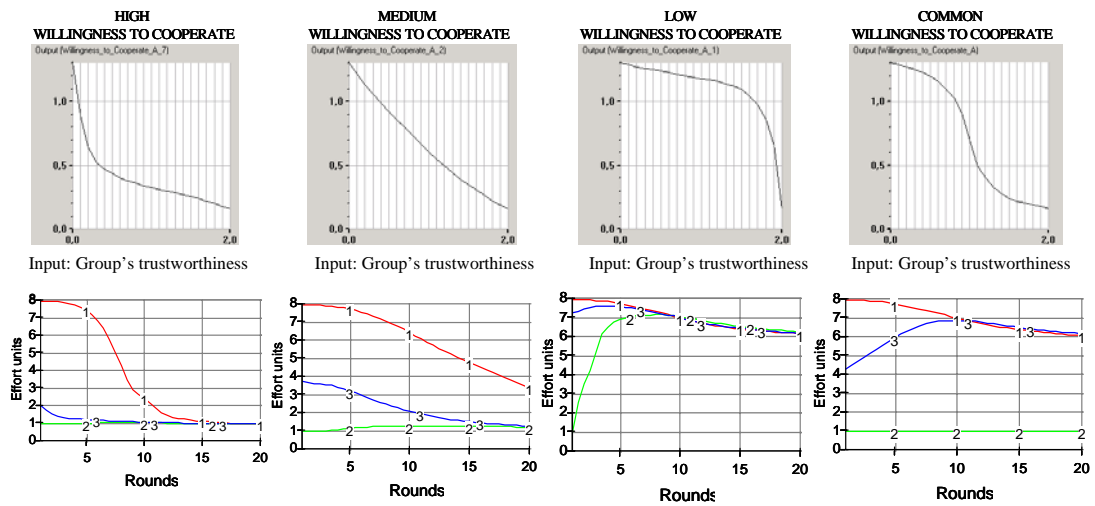
Figure 8. Sensitivity analysis of willingness to cooperate function
