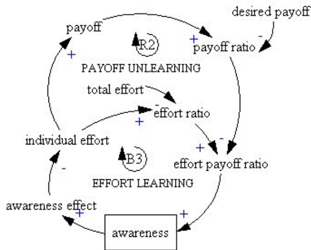
Figure 5. Awareness building loops
