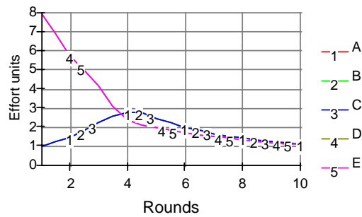
Figure 10. Simulation of a reciprocity norm of Ostrom (1998)
