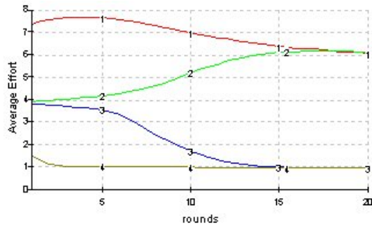
Figure 13. Path dependence pattern: simulations with different initial values of trust
