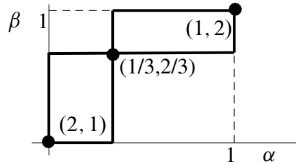
Figure 2.2. Nash equilibria in the Battle of the Sexes
