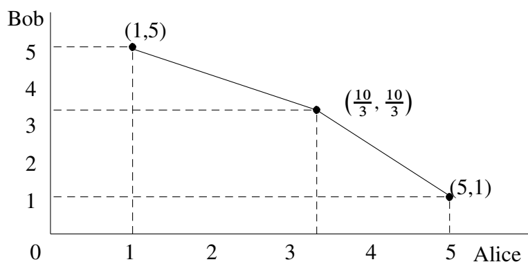
Figure 2.4. Alice, Bob, and the choreographer
