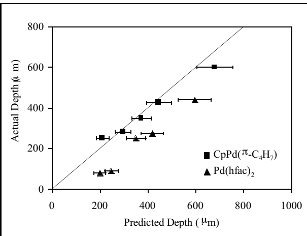
Figure 5. Parity plot comparing the actual depth of the Pd deposit to model predictions.
