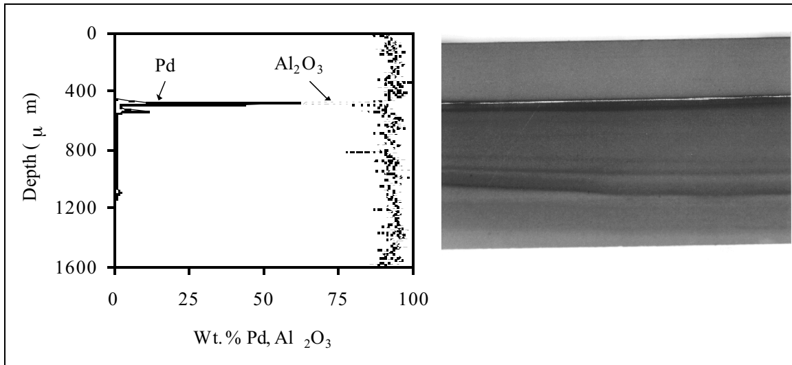
Figure 3. EPMA and Optical Microscopy Analysis of a thin Pd membrane deposited within an Al 2 O 3 support.
