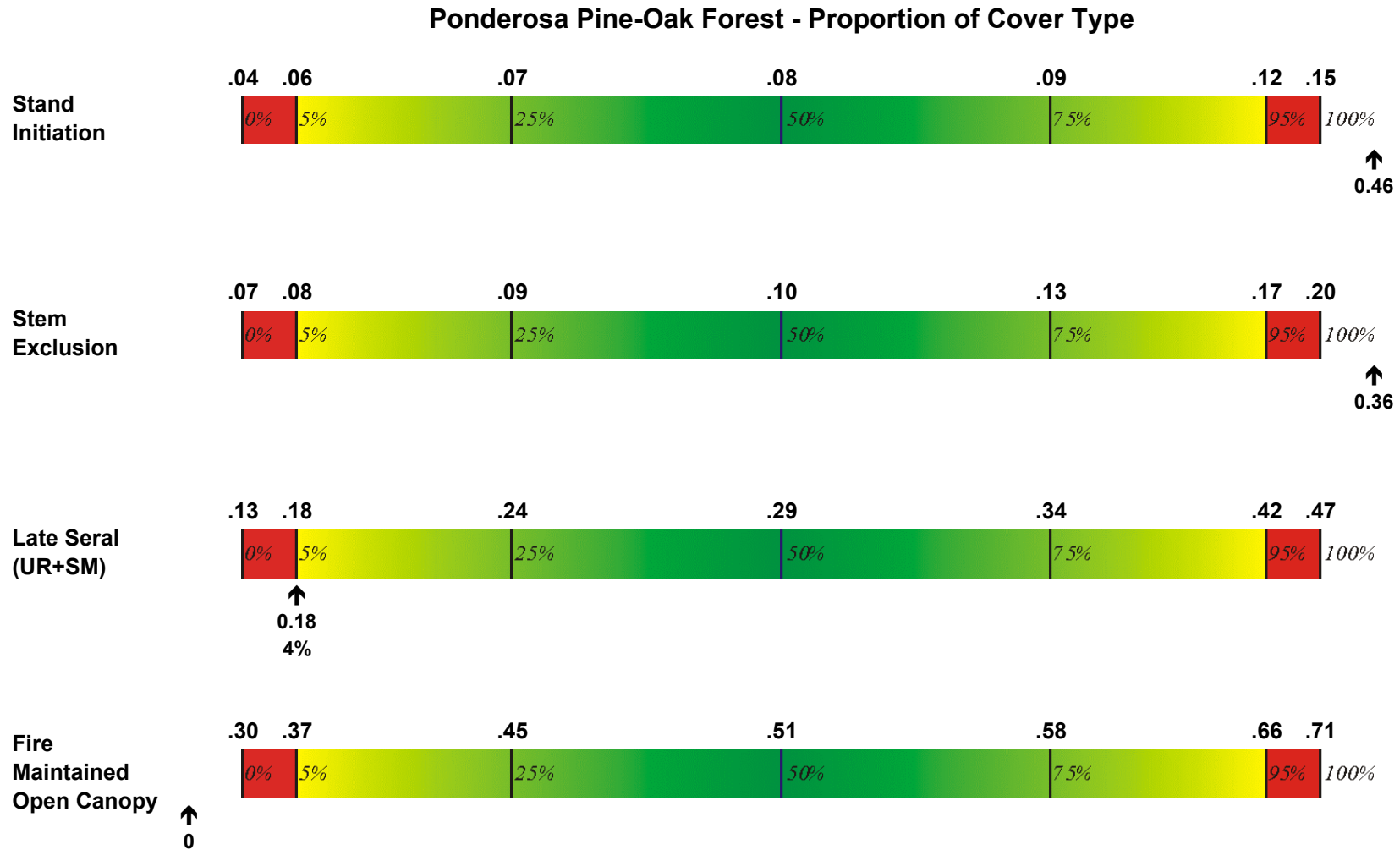
Figure. Simulated historic range of variability (HRV) in seral stage (i.e., Condition class) distribution of ponderosa pine-oak forest (37,976 ha) over five 800-year simulations on the Uncompahgre Plateau Landscape, Colorado. The range of variability is shown as a color gradient bar and is subdivided into 5, 25, 50, 75, and 95 percentiles of the distribution. Bold numbers above the bar represent the proportion of the cover type in the corresponding condition class at the specified percentile. The bold arrow denotes the condition of the current landscape.
