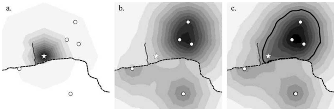
Figure 2. Examples of the resistant-kernel estimator at three scales in a landscape with a focal pool (star), five neighboring pools (circles), and two roads: (a) local scale, showing connectivity to upland habitat from the focal pool; (b) neighborhood scale, showing the probability of the focal pool receiving dispersing animals from each neighboring pool; and (c) regional scale, with dark outline indicating pools that are interconnected by a specified level of dispersal. Darker shading indicates greater connectivity at each scale.
