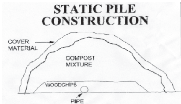
Figure 1. Diagram of a static pile construction with a perforated pipe insert.
